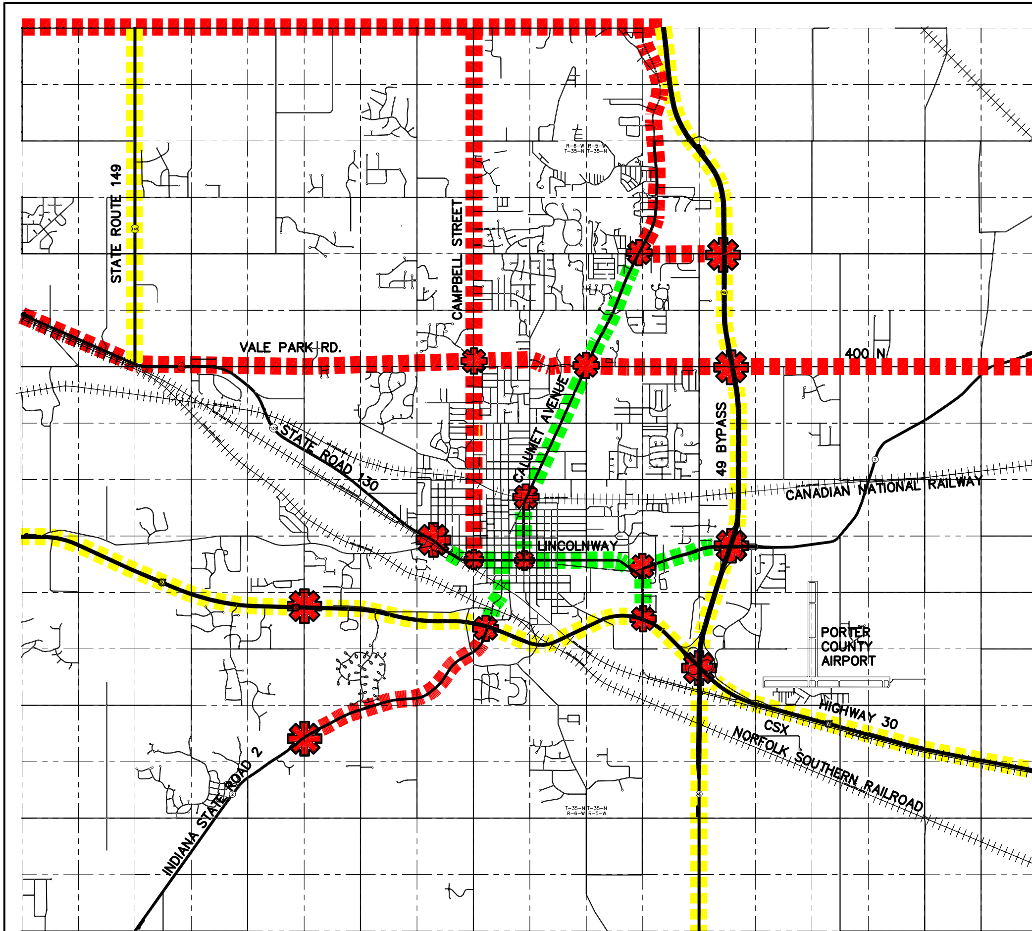
Figure 8: PROPOSED CORRIDOR DESIGN PLAN
